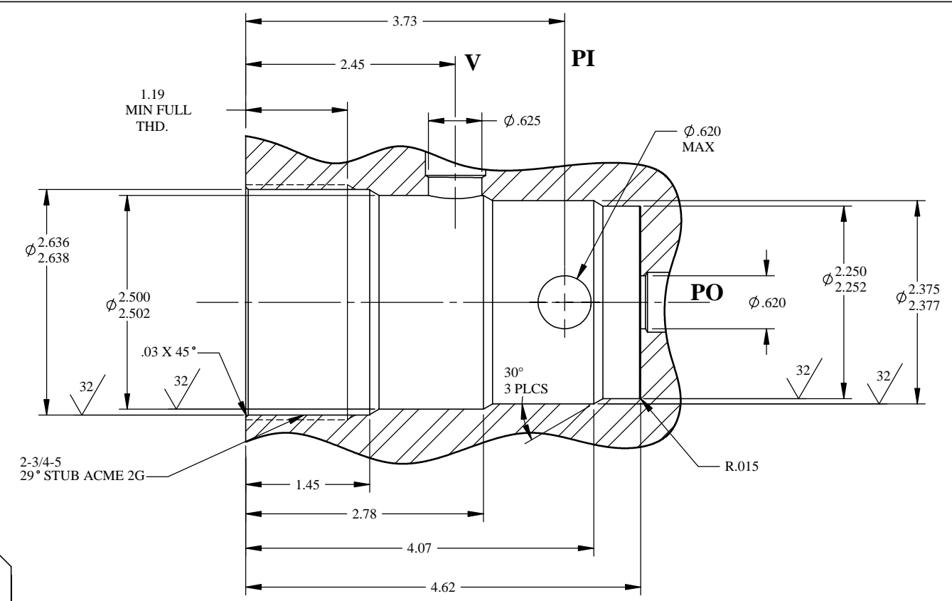
CAVITY DETAIL
