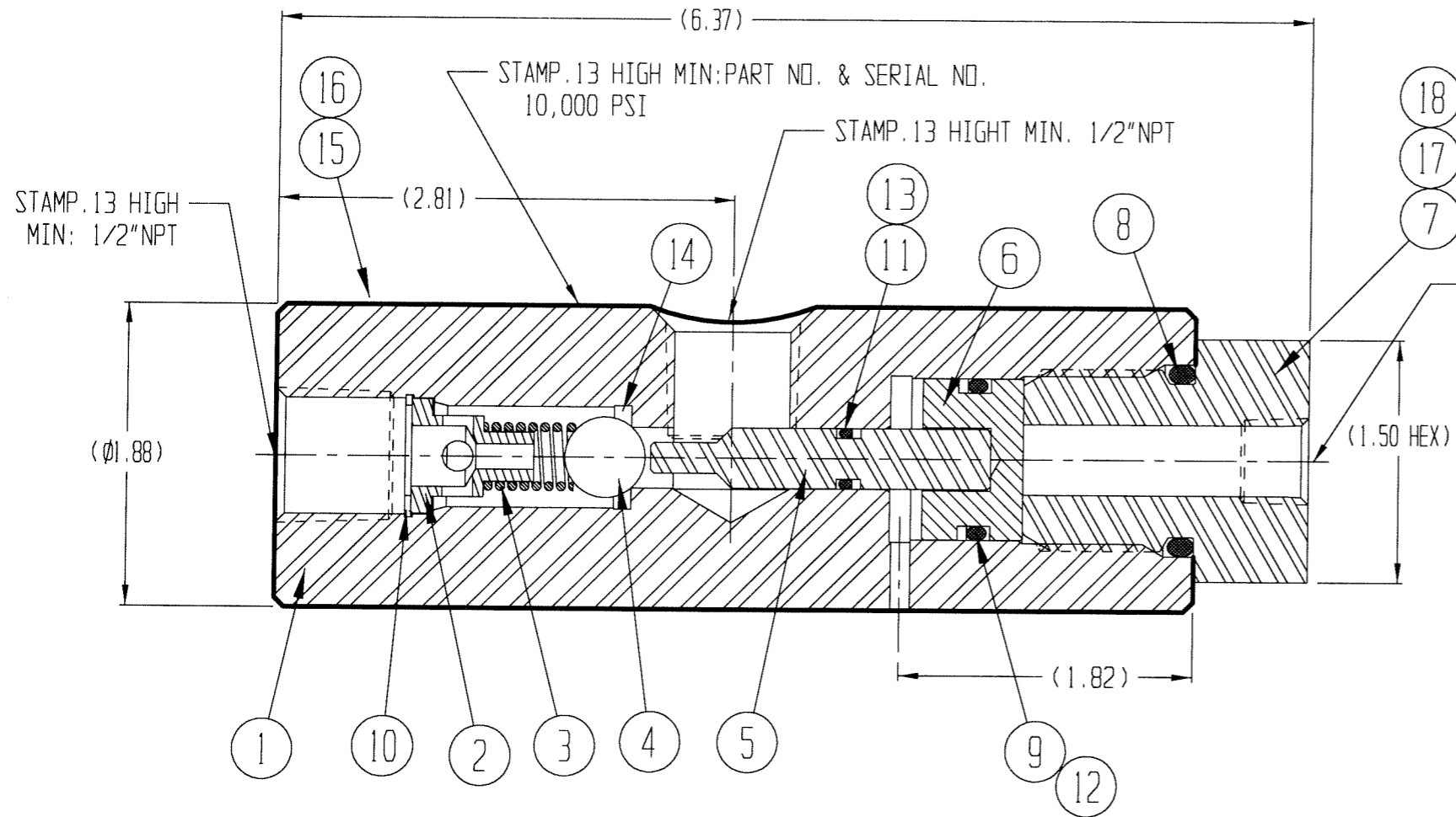
SECTION VIEW
